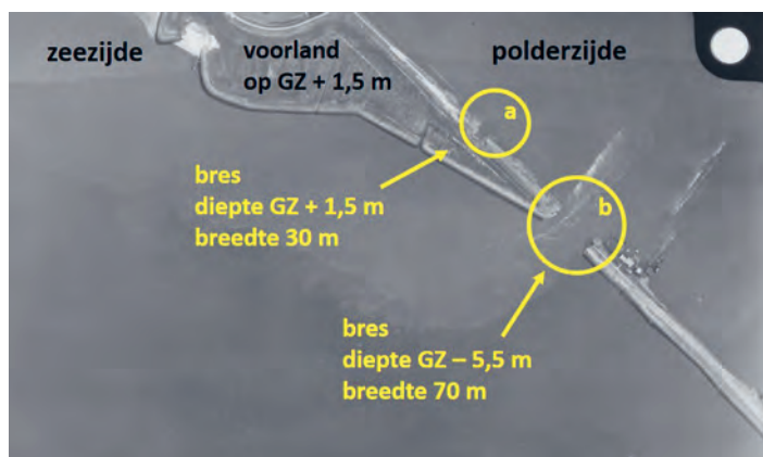
Afb. 2 Dijkdoorbraken in 1953 in de polder Oudenhooen (opname 7 februari). Z. Zhu e.a., 'Historic storms and the hidden value of coastal wetlands for nature-based flood defence', Nature Sustainability 3 (2020) 853-862.
